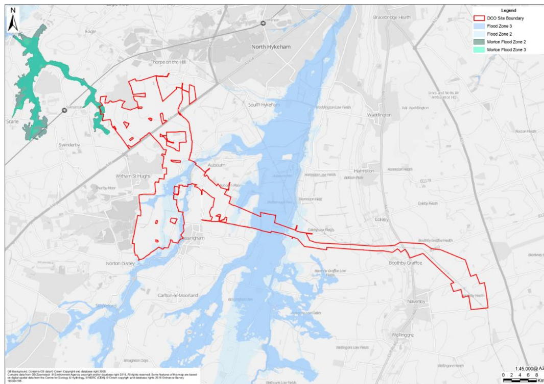
Plate 3-1 Fluvial flood risk map
